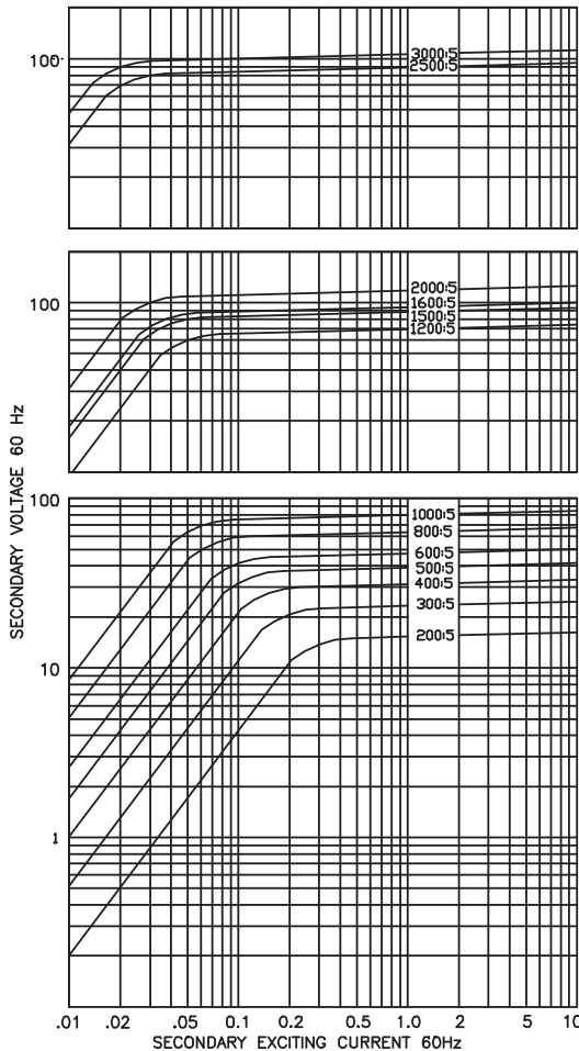
EXCITATION CURVE
