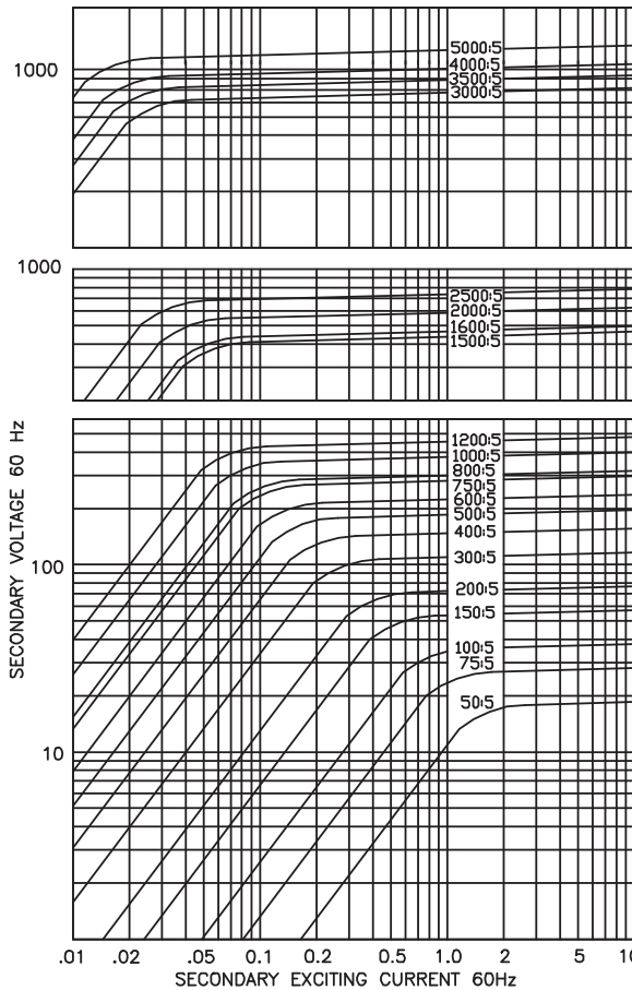
EXCITATION CURVE
