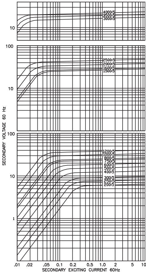
EXCITATION CURVE
